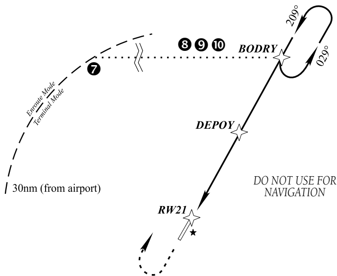
Figure 6-27 Terminal Mode
